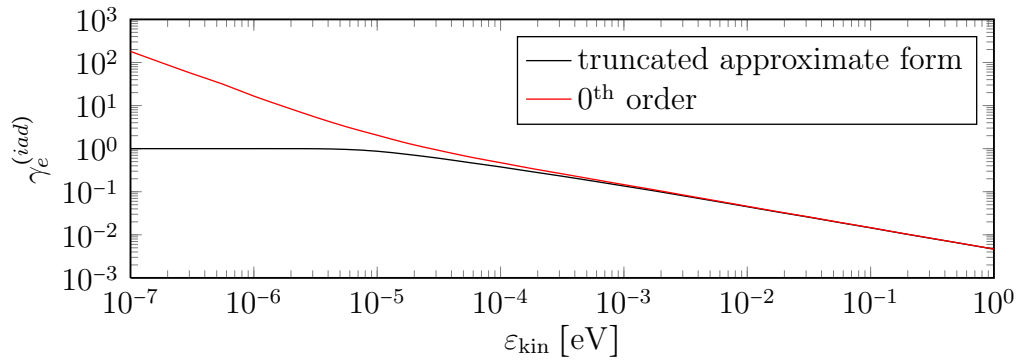
Figure 4.2: Comparison of the secondary electron emission coefficient \gamma_e^{(iad)} computed from the truncated approximate form (3.68) (black line) and the zeroth order of (3.62b) (red line) which is obtained by dropping the \sigma -terms. The graphs were calculate for an aluminum surface without Coulomb screening and a nitrogen molecule in the perpendicular orientation.
