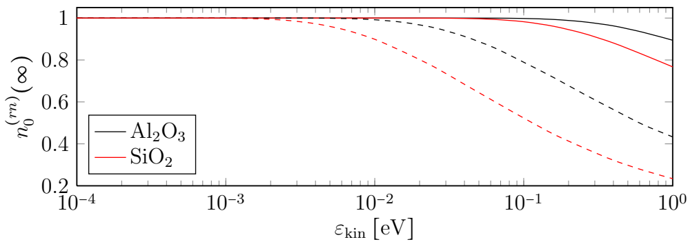
Figure 5.4: Kinetic energy dependence of the final occupation of the projectile's ground state level n_0^{(rn)}(\infty) due to the resonant neutralization of N_2^+(^2\Pi_u) on Al_2O_3 (black lines) and SiO_2 (red lines). The plot shows curves for the parallel (solid lines) as well as the perpendicular (dashed lines) molecule orientation. The results were calculated using Eq. (3.134).
