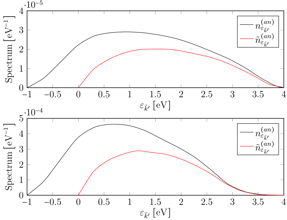
Figure 5.2: Final energy spectrum of the Auger electrons due to the neutralization of \text{He}^+(^2S_{1/2}) on \text{Al}_2\text{O}_3 at a kinetic energy of 50 meV. Here n_{\varepsilon_{\vec{k}'}}^{(an)} and \tilde{n}_{\varepsilon_{\vec{k}'}}^{(an)} refer to the internally excited electrons within the surface (black lines) and the electrons capable of escaping the surface (red lines), respectively. The upper panel shows the results obtained using the turning point z_0 \approx 3.6 a_B emerging from (2.53) with the parameters due to Bonini et al. [13] while in the lower panel we employed the turning point z_0 = 1.2 \cdot 10^{-10} \text{ m} \approx 2.27 a_B which was suggested by Modinos and Easa [96] . Note that the angularity of the curves is a consequence of our numerical tabulation scheme and could be removed by allowing for a larger computation time.
