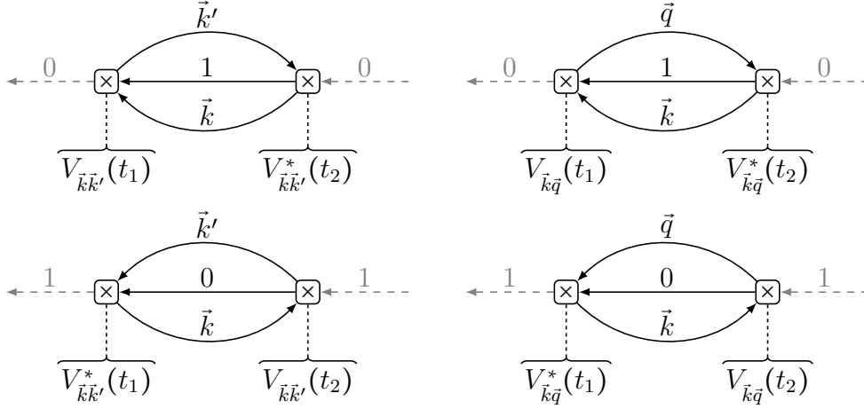
Figure 3.1: Second-order self-energy diagrams of the molecular ground state level (upper two diagrams) and the excited level (lower two diagrams). In both rows of this figure the left diagram is due to the direct de-excitation channel (1.3) while the right one pertains to the indirect reaction (1.2). Note that the gray dashed lines merely represent the diagram's connectors and do not belong to the actual self-energies.
