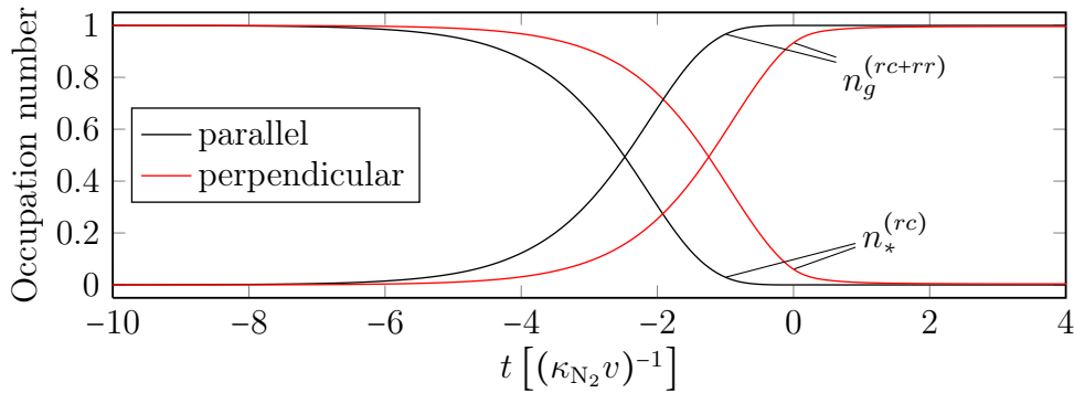
Figure 4.9: Time evolution of the molecular fractions n_*^{(rc)} and n_g^{(rc+rr)} pertaining to the metastable state and the ground state molecule, respectively. The figure shows data for the parallel (black lines) and perpendicular (red lines) orientation on an \text{Al}_2\text{O}_3 surface at a kinetic energy of 50 meV. The curves were obtained by employing Eqs. (3.92a) and (3.97), respectively, while only considering the natural decay channel.
