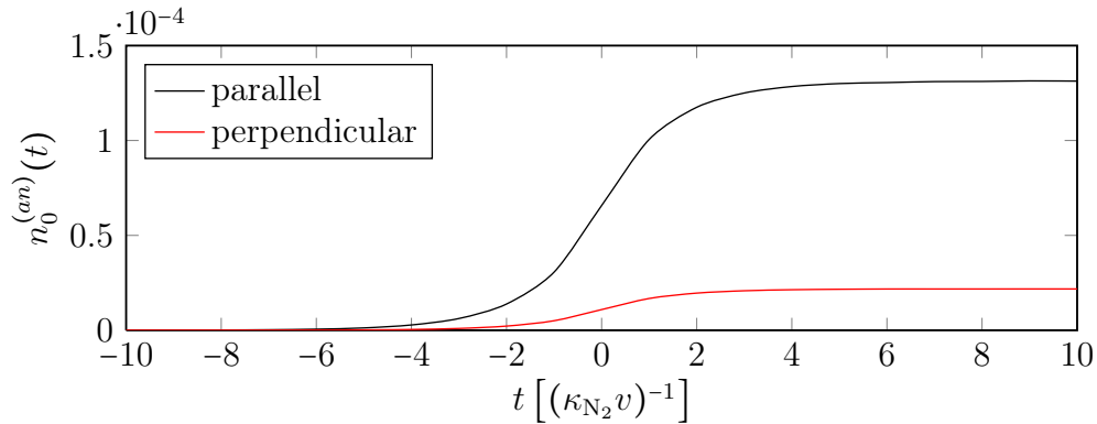
Figure 5.1: Time dependence of the occupation of the projectile level n_0^{(an)} due to the Auger neutralization of N_2^+(^2\Pi_u) on a CaO surface. Separate graphs are shown for the parallel (black line) and perpendicular (red line) orientation. The results were calculated from Eq. (3.134) at a kinetic energy of 50 meV.
