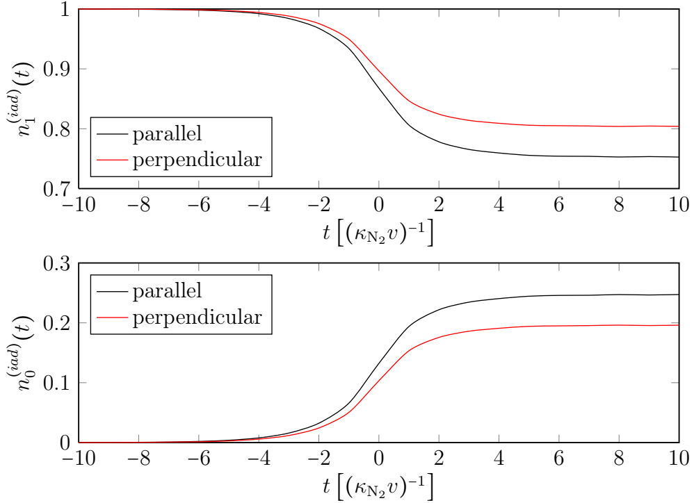
Figure 4.4: Time evolution of the occupancies of the excited molecular level (upper panel) and the ground state level (lower panel) for parallel (black lines) and perpendicular (red lines) molecule orientation on an aluminum surface. The kinetic energy of the incident molecule was fixed to 50 meV. Moreover, the curves were calculated from (3.65a) and (3.65b), respectively, while neglecting Coulomb screening effects. Note that here the time is measured in the atomic units of (4.9). Thus, a time difference of \Delta t = 1 corresponds to the motion of the molecule over a distance of \Delta z = a_B/2 .
