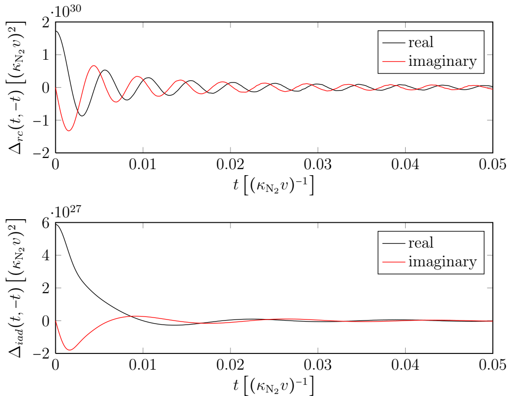
Figure 4.12: Variation of the real (black lines) and imaginary (red lines) part of \Delta_{rc}(t_1, t_2) (upper panel) and \Delta_{iad}(t_1, t_2) (lower panel) as calculated from (4.22) and (4.10) along the anti-diagonal t_1 = -t_2 = t . The results hold for a diamond surface and an \text{N}_2(^3\Sigma_u^+) molecule with its axis aligned perpendicular to the surface at a kinetic energy of 50 meV. The behavior for negative time arguments t is omitted since the real (imaginary) part of both functions is symmetric (anti-symmetric) with respect to the time diagonal.
