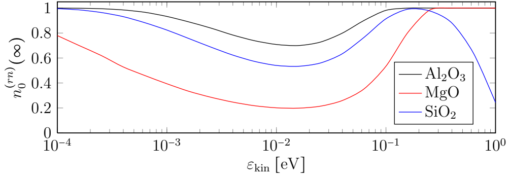
Figure 5.5: Kinetic energy dependence of the final occupation of the projectile's ground state level n_0^{(rn)}(\infty) due to the resonant neutralization of \text{Ar}^+(^2P_{3/2}) on \text{Al}_2\text{O}_3 (black line), \text{MgO} (red line) and \text{SiO}_2 (blue line). The curves were calculated from (3.134).
