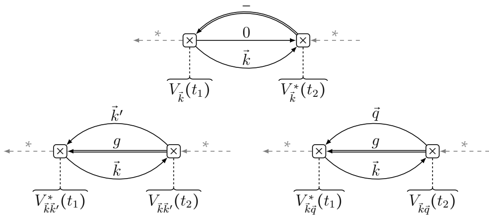
Figure 3.4: Second-order self-energy diagrams of the metastable state in non-crossing approximation. The upper diagram depicts the component of \Sigma_{**} due to resonant electron capture whereas the lower left and right diagrams constitute the direct and indirect Auger term, respectively. Here again a double line symbolizes a full propagator.
