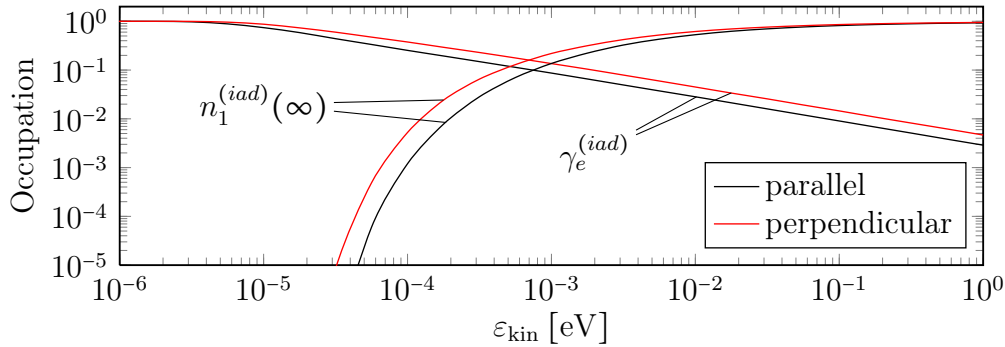
Figure 4.1: Secondary electron emission coefficient \gamma_e^{(iad)} and final occupancy of the excited molecular level n_1^{(iad)}(\infty) in parallel (black lines) and perpendicular (red lines) molecule orientation over the molecule's kinetic energy \varepsilon_{\text{kin}} . The curves were calculated for an aluminum surface without Coulomb screening using the formulas (3.65b) and (3.68), respectively.
