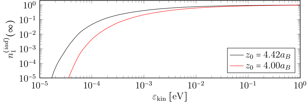
Figure 4.6: Comparison of the final occupancy of the excited molecular level n_1^{(iad)}(\infty) for two different values of the turning point z_0 . The curves were computed for a tungsten surface in the perpendicular orientation by means of (3.65b). The effect of screening was not included.
