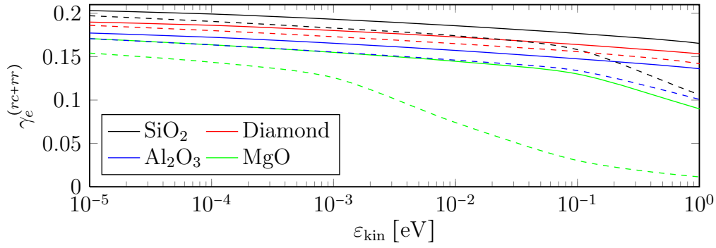
Figure 4.11: Secondary electron emission coefficient \gamma_e^{(rc+rr)} for several dielectric surface materials plotted against the molecule's kinetic energy \varepsilon_{\text{kin}} . The individual materials are encoded in different colors and in each case two curves are depicted. The solid one corresponds to the parallel molecule orientation whereas the dashed one identifies the perpendicular molecule orientation. All of the results were obtained from Eq. (3.105).
