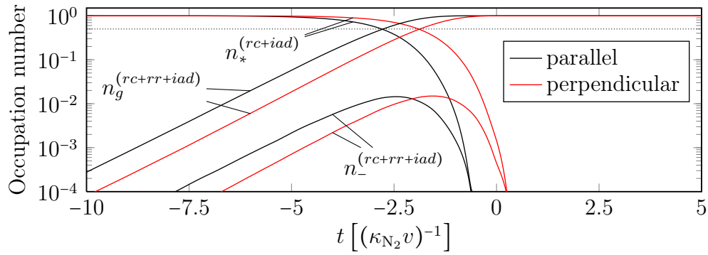
Figure 4.13: Transient occupation of the pseudo-particle levels of the ground state molecule n_g^{(rc+rr+iad)} , the metastable molecule n_*^{(rc+iad)} and the negative ion n_-^{(rc+rr+iad)} in parallel (black lines) and perpendicular (red lines) orientation for a diamond surface. The molecule’s kinetic energy was fixed to 50 meV and the dotted line represents half filling of the respective level. The curves were calculated from Eqs. (3.94), (3.96) and (3.97), respectively.
