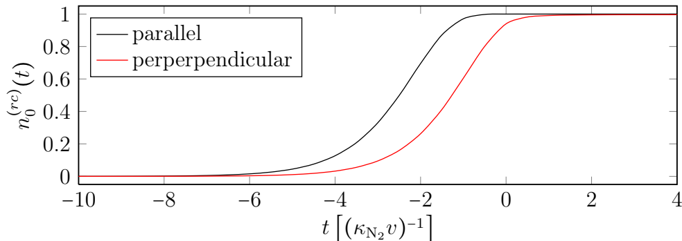
Figure 4.7: Time evolution of the occupation of the molecular ground state level n_0^{(rc)} in front of an \text{Al}_2\text{O}_3 surface for parallel (black line) and perpendicular (red line) molecule orientation. The curves were calculated from (3.93a) and (3.92a) for a kinetic energy of 50 meV.
