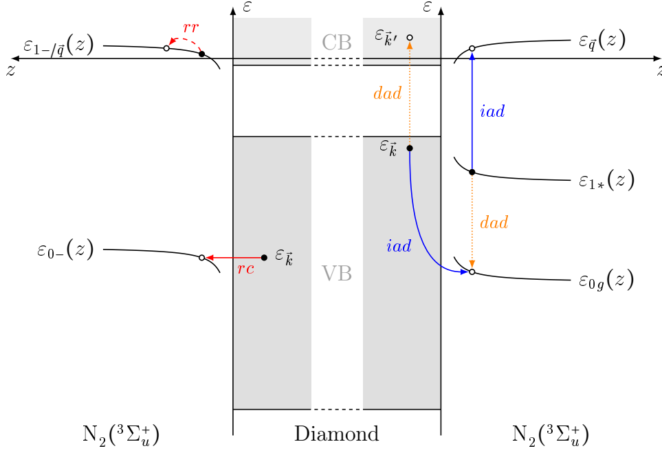
Figure 1.1: Schematic illustration of the different de-excitation channels of N_2(^3\Sigma_u^+) on a diamond surface. Occupied electronic states are indicated by \bullet while empty states are marked with \circ . Furthermore, the drawing is to scale in terms of energy units and VB and CB denote the valence and conduction band, respectively. The left panel depicts the RCT reaction (1.1) embracing the subprocesses of resonant capture ( rc ) and resonant release ( rr ) of an electron. The latter transition is drawn with a dashed line because the electron emission actually occurs at the same z -position and, hence, at the same energy. Consequently, the emitted electron will only reach the shown location over time. Furthermore, the right panel shows the reactions of indirect Auger de-excitation ( iad ) and direct Auger de-excitation ( dad ), Eqs. (1.2) and (1.3). The direct Auger transition is drawn with a dotted line as it is spin-blocked for the N_2(^3\Sigma_u^+) -state. Note that the projectile levels' energies and image shifts are determined in terms of the removal of an electron and, hence, depend on the molecular state formed through the transitions (see Table A.3 and Sec. 2.2.4). For clearness in the above figure the level energies \varepsilon_0 and \varepsilon_1 , thus, carry additional subscripts g , * and - denoting the respective level's energy in the molecular ground state N_2(^1\Sigma_g^+) , the metastable molecule N_2(^3\Sigma_u^+) and the negative ion N_2(^2\Pi_g^-) .
