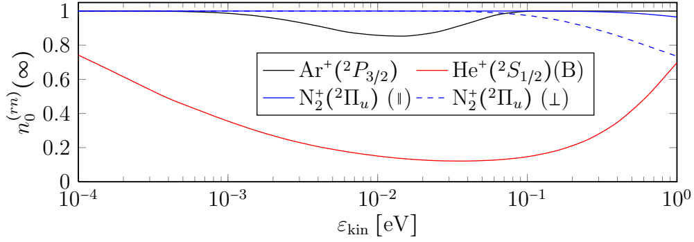
Figure 5.6: Kinetic energy dependence of the final occupation of the projectile's ground state level n_0^{(rn)}(\infty) due to the isolated resonant neutralization of \text{He}^+(^2S_{1/2}) , \text{Ar}^+(^2P_{3/2}) and \text{N}_2^+(^2\Pi_u) on a diamond surface. The curves were calculated from (3.134). Note that for \text{He}^+(^2S_{1/2}) only the turning point due to Bonini et al. [13] (B) was considered since the z_0 -value proposed by Modinos and Easa [96] only applies to \varepsilon_{\text{kin}} = 50 \text{ meV} . Moreover, as before, \parallel and \perp indicate the parallel and perpendicular orientation of the \text{N}_2^+(^2\Pi_u) ion.
