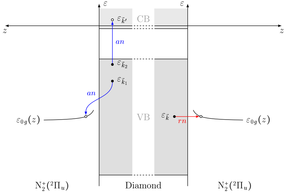
Figure 1.2: Schematic representation of the Auger and resonant neutralization channels for the special case of N_2^+(^2\Pi_u) on a diamond surface. The figure is to scale in terms of energy units. The left panel shows the Auger neutralization ( an ) reaction (1.4) whereas the right panel depicts the resonant neutralization ( rn ) channel (1.5). As the neutralization ends up in the molecular ground state N_2(^1\Sigma_g^+) , the projectile level's energy is \varepsilon_{0g} in both reaction channels (see also the caption of Fig. 1.1).
