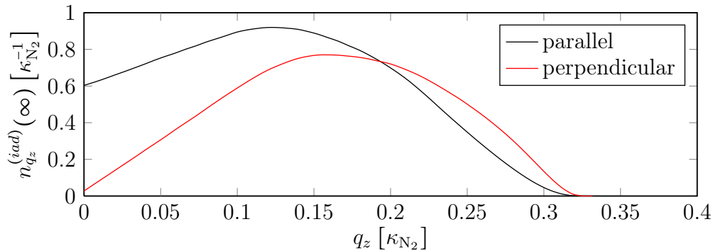
Figure 4.3: Distribution of emitted electrons over the z -component of \vec{q} for an aluminum surface in parallel (black line) and perpendicular (red line) orientation. The curves were computed from (3.54b) by dropping the \sigma -terms and integrating over the lateral wave vector dependence. The effect of Coulomb screening was not included. Note that q_z is denoted in units of \kappa_{N_2} (see Eq. (2.34)) and only the region q_z \geq 0 is shown since wave vectors pointing in the negative z -direction traverse into the solid and, thus, cannot escape the surface.
