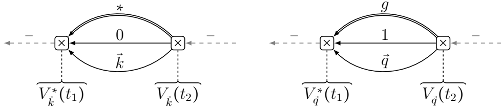
Figure 3.3: Second-order self-energy diagrams of the negative ion state in non-crossing approximation. Here the left diagram represents the contribution to \Sigma_{--} due to resonant electron capture while the right diagram pertains to the surface-induced resonant electron emission. As before, a double line indicates a full propagator.
