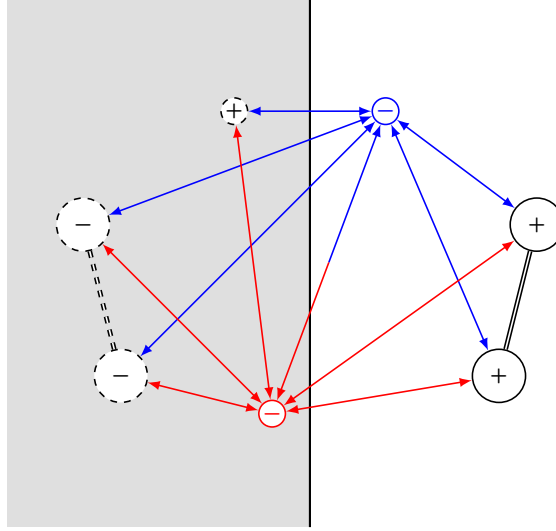
Figure 2.7: Exemplary distribution of actual (solid circles) and image (dashed circles) charges for a neutral diatomic molecule in front of a metallic or dielectric surface. The solid is located on the left-hand side and positive and negative charges have been marked with + and -, respectively. In the depicted situation the blue electron belongs to the projectile and resides outside the surface while the red electron occupies a band state inside the solid. The latter electron does, thus, not generate an image charge by itself. On the projectile side the positive nucleus charges result from the screening of the actual core charges by the passive electrons on the projectile. The relevant interactions between the electrons and the various real and image charges are marked with arrow lines.
