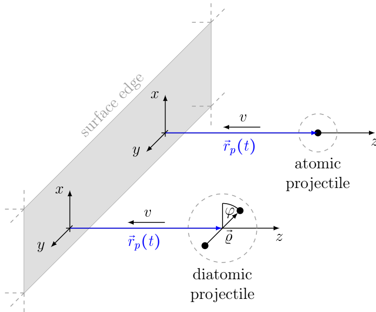
Figure 2.5: Schematic illustration of the collision geometry for atomic and diatomic projectiles. Here \vec{r}_p denotes the projectile's center of mass and v represents its velocity. Moreover, for the diatomic case \varrho denotes the molecule's bond length and \varphi is the angle between the z -axis of the molecular reference frame and the surface. Note that the corresponding angle for atomic particles is not shown in order not to overload the drawing. In addition, the orientation of the projectile reference frame can be expected to play a minor part for mononuclear particles.
