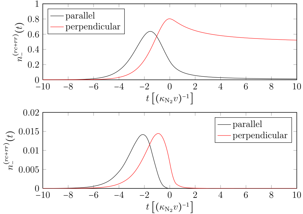
Figure 4.8: Fraction of negative ions versus time for the surface-induced decay process (upper panel) and the natural decay reaction (lower panel) in front of an \text{Al}_2\text{O}_3 surface at a molecular kinetic energy of 50 meV. The black lines represent the parallel orientation whereas the red lines denote the perpendicular orientation. The results were calculated from Eq. (3.96).
