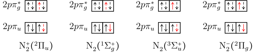
Figure 2.3: Occupation of the 2p\pi_u and 2p\pi_g^* orbitals in the different molecular states of nitrogen. Empty electronic states are indicated by the dashed arrows \uparrow and \downarrow , respectively. Furthermore, electronic orbitals whose occupation has to be changed in order to switch between the depicted states of the molecule have been marked in red. Note that for the negative ion the depicted configuration is not the only possible arrangement. It does, however, emerge when an electron is attached to the metastable state which is the process under consideration in this work (see Eq. (1.1)).
