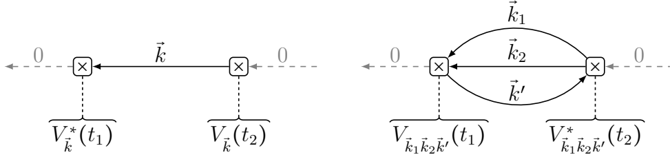
Figure 3.6: Diagrammatic representation of the self-energy \Sigma_{00} up to second order. The left diagram shows the component due to resonant neutralization which for the isolated resonant channel represents the exact self-energy. The right diagram, on the other hand, depicts the second-order self-energy term due to the Auger neutralization channel.
