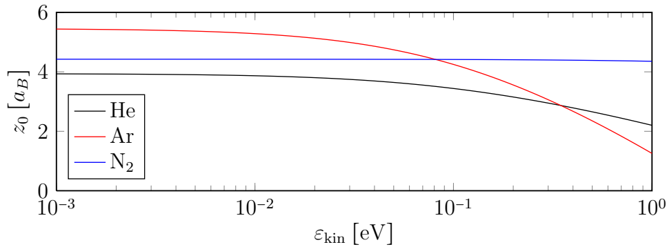
Figure 2.6: Variation of the turning point z_0 with the projectile’s kinetic energy \epsilon_{\text{kin}} for He, Ar and N 2 . The values of z_0 were calculated from the Morse potential (2.52) by means of (2.53) using the parameters listed in Appendix A.
