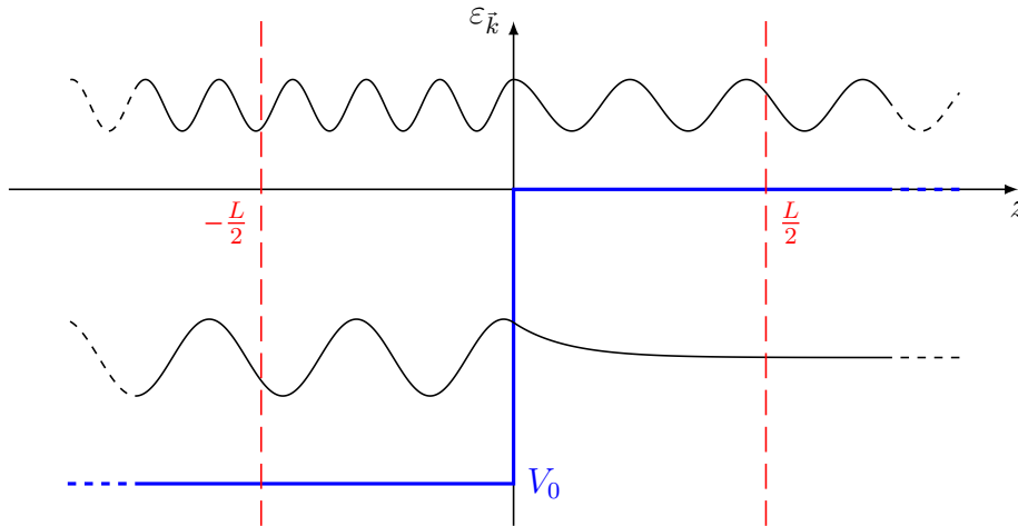
Figure 2.1: Square potential well model used for the calculation of the solid's wave functions. The vertical axis represents the energy scale while the horizontal axis denotes the distance from the surface edge. On the solid side the well has a depth of V_0 whereas outside the surface the potential vanishes. The dashed red lines mark the limits of the box normalization volume [-L/2, L/2]^3 on the z -axis. Also indicated here is the schematic form of the wave function for a bound and an internally excited electron.
