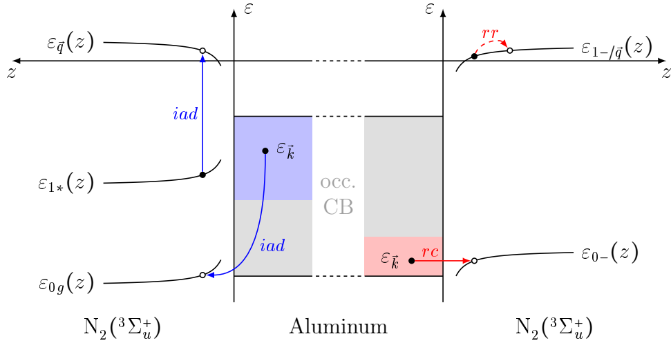
Figure 4.17: Band structure of aluminum together with the active zones for indirect Auger de-excitation (purple) and two-step resonant de-excitation (light red). The active areas were calculated from (4.40) and (4.41) using a maximum image shift of 2 eV and an additional near-resonance shift of \pm 1 eV. Note that only the occupied portion of the conduction band (occ. CB) is shown.
