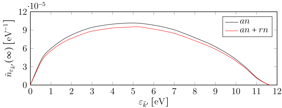
Figure 5.7: Final energy spectrum of the escaped Auger electrons due to the isolated Auger neutralization ( an , black line) and the two channel neutralization ( an + rn , red line) of \text{He}^+(^2S_{1/2}) on a diamond surface. The results were obtained for a kinetic energy of 50 meV with the turning point due to Bonini et al. [13] . Note that the angularity of the curves is a consequence of our numerical tabulation scheme and could be removed by allowing for a larger computation time.
