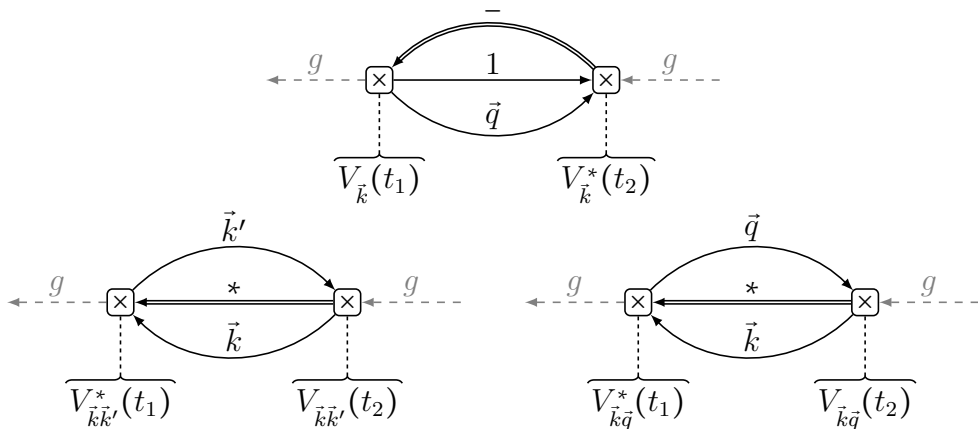
Figure 3.5: Second-order self-energy diagrams of the ground state in non-crossing approximation. Here the upper diagram pertains to the surface-induced resonant electron emission while the lower left and right diagrams embrace the contributions to \Sigma_{gg} due to direct and indirect Auger de-excitation, respectively. Like before, a double line stands for a full propagator.
