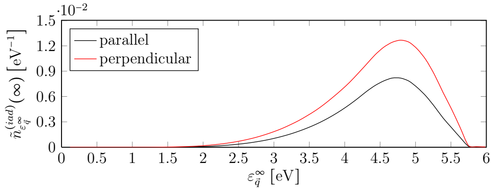
Figure 4.5: Final energy spectrum of the escaped electrons in parallel (black line) and perpendicular (red line) orientation. The kinetic energy of the incident molecule was fixed to 50 meV. Moreover, the graphs were calculated for an aluminum surface without Coulomb screening by means of (4.35) and (3.61b).
