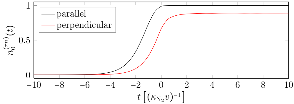
Figure 5.3: Time dependence of the occupation of the projectile level n_0^{(rn)}(t) due to the resonant neutralization of N_2^+(^2\Pi_u) on an Al_2O_3 surface. Separate graphs are shown for the parallel (black line) and perpendicular (red line) orientation. The results were calculated from Eq. (3.134) for a kinetic energy of 50 meV.
