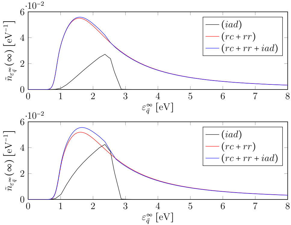
Figure 4.15: Energy spectrum of the escaped electrons in parallel (upper panel) and perpendicular (lower panel) orientation as calculated from (3.106b) for a diamond surface at a kinetic energy of 50 meV. In both panels the black line specifies the isolated spectrum of indirect Auger de-excitation ( iad ), the red line denotes the isolated spectrum due to the two-step resonant reaction ( rc + rr ) and the blue line represents the combined two-channel spectrum ( rc + rr + iad ). Note that the angularity of the Auger spectrum is a consequence of the tabulations performed in our numerical scheme and could be avoided by choosing a finer grid (see also Appendix E).
