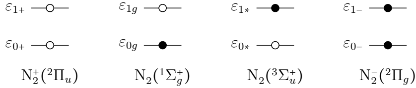
Figure 2.4: Effective two-level system and its relation to the different states of the nitrogen molecule. Occupied states are indicated by \bullet whereas empty states are marked with \circ . Furthermore, \varepsilon_0 and \varepsilon_1 denote the energies of the levels 0 and 1 and the indices + , g , * and - characterize the respective molecular state.
