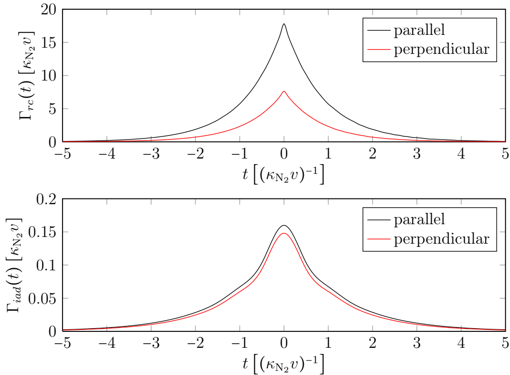
Figure 4.14: Variation of the rates of resonant electron capture \Gamma_{rc} (upper panel) and indirect Auger de-excitation \Gamma_{iad} (lower panel) for the parallel (black lines) and perpendicular (red lines) molecule orientation. The curves were calculated from (3.87a) and (3.87d) for a diamond surface at a projectile energy of 50 meV.
