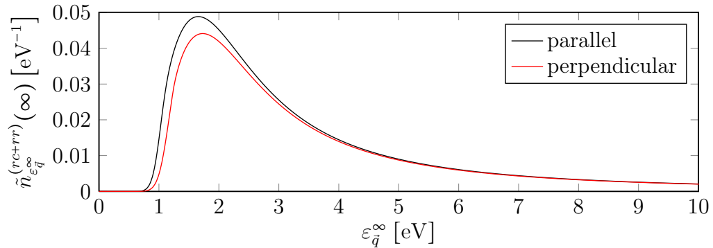
Figure 4.10: Final spectrum of escaped electrons for an \text{Al}_2\text{O}_3 surface calculated from Eq. (3.106b) in parallel (black line) and perpendicular (red line) orientation. The molecule’s kinetic energy was fixed to 50 meV and only the natural decay process was taken into account.
