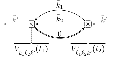
Figure 3.7: Dressed second-order self-energy of the excited surface states \vec{k}' . The full propagator of the projectile level is indicated by a double line.
