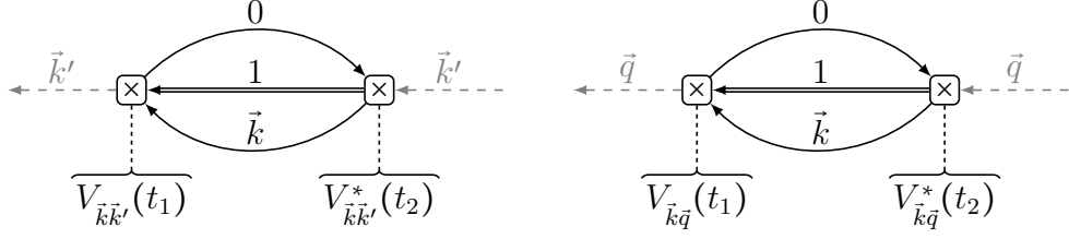
Figure 3.2: Second-order diagrammatic representation of the dressed self-energies \Sigma_{\vec{k}'\vec{k}'}^K (left panel) and \Sigma_{\vec{q}\vec{q}}^K (right panel). The full propagator of the excited level G_{11} is indicated by a double line.
