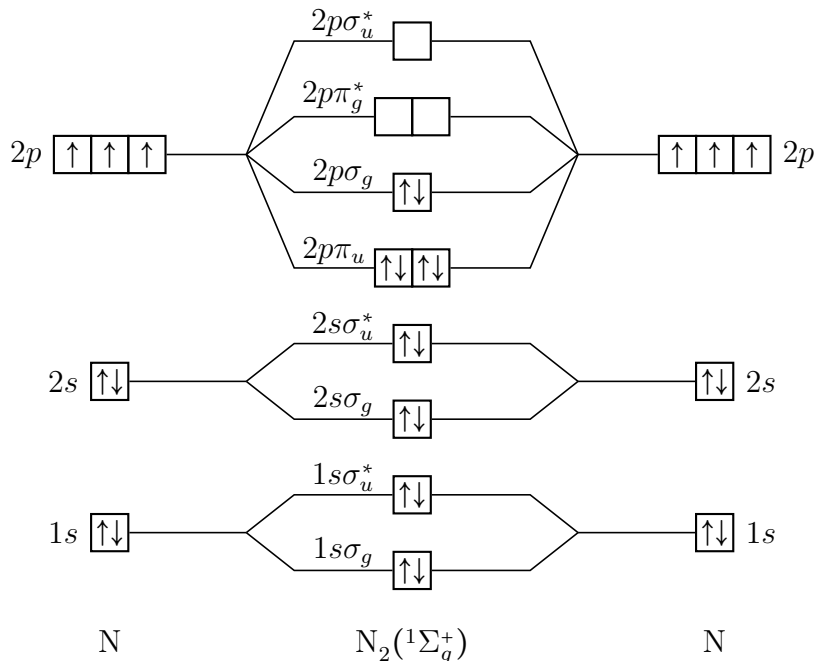
Figure 2.2: Molecular orbitals of N_2 as constructed from atomic nitrogen orbitals by means of the LCAO technique. Within the LCAO framework various different notation conventions for the designation of molecular orbitals have been established. In the above figure we employed a mixture of the styles used in Refs. [8] and [46]. Moreover, as usual, electrons with spin \pm\frac{1}{2} are indicated by \uparrow and \downarrow , respectively. Note that the \sigma -orbitals correspond to a magnetic quantum number of m = 0 whereas the \pi -orbitals are twofold degenerate in m involving m = \pm 1 . Furthermore, the depicted occupation of the molecular orbitals represents the ground state N_2(^1\Sigma_g^+) .
